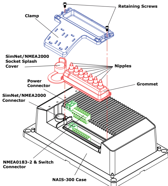
Figure 2.2 - NAIS-300 assembly
